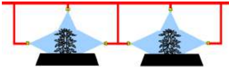
Figure 3. Use one nozzle over the row up to 8 inches, then change to three nozzles for optimum coverage of the tomato plant.
